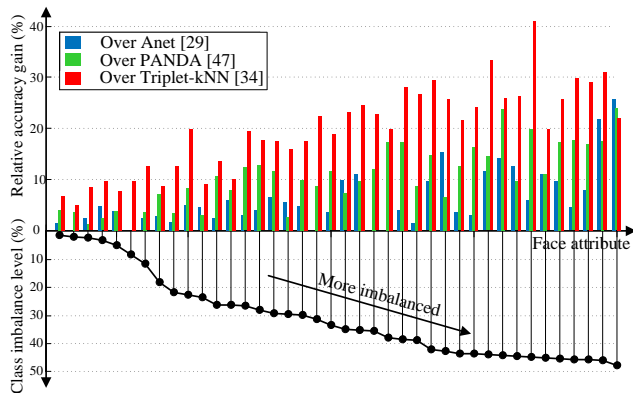
Figure 4. Relative accuracy gains over competitors on the sorted 40 face attributes in Table 2.
