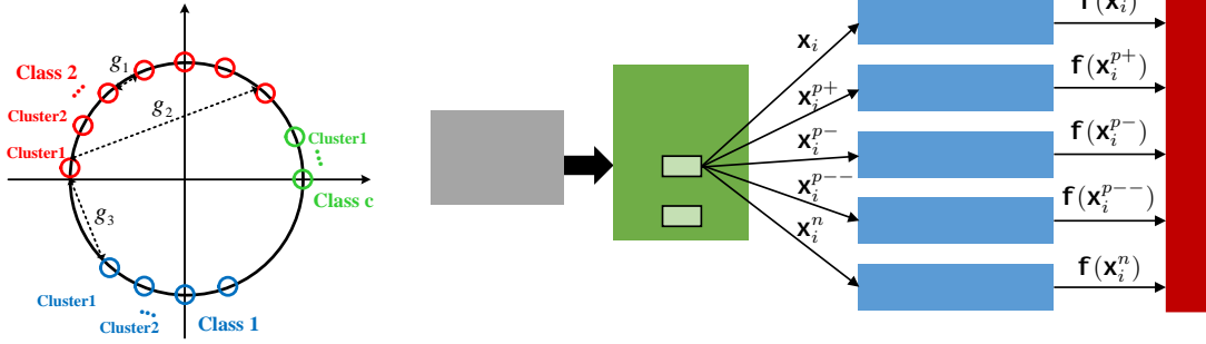
Figure 2. (a) Feature distribution in 2D space and the geometric intuition of margins. (b) Our learning network architecture.
